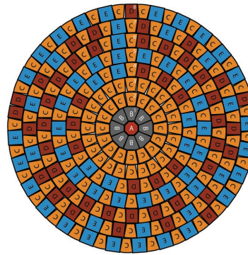
Kit Diameter 7'-10" [94"]
