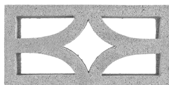
STARFIRE 6 x 8 x 16 | 29 LBS 48% VOID PER UNIT
