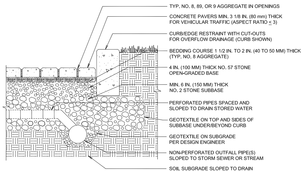
Figure 6. Partial infiltration through the soil subgrade. Perforated pipes can be raised above the soil subgrade to drain water from higher depth rainstorms. Smaller storms which often contain higher pollutant concentrations can be captured below the perforated pipes, stored and infiltrated.
