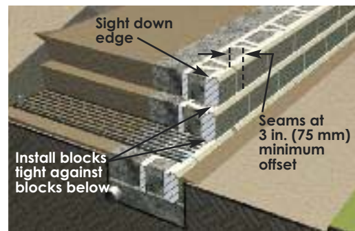
Install additional courses.
