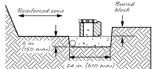
Reinforced Wall Base Course Cross Section.
