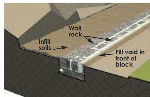
Install wall rock.
