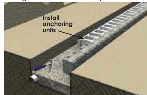
Install AB Fieldstone anchoring units.
