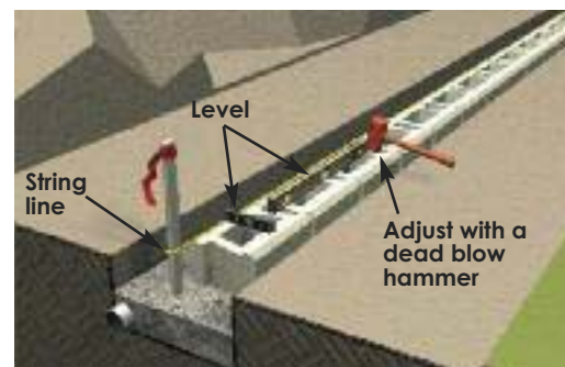
Install base course.
