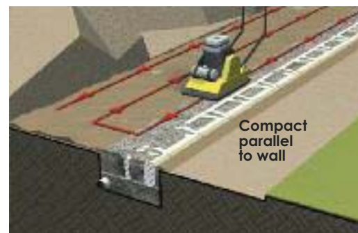
Compact wall rock and backfill soils.
