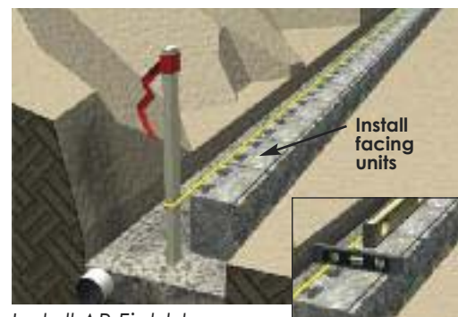
Install AB Fieldstone facing units. Level and adjust.
